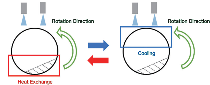
Figure 3-3: Cooling Mechanism
