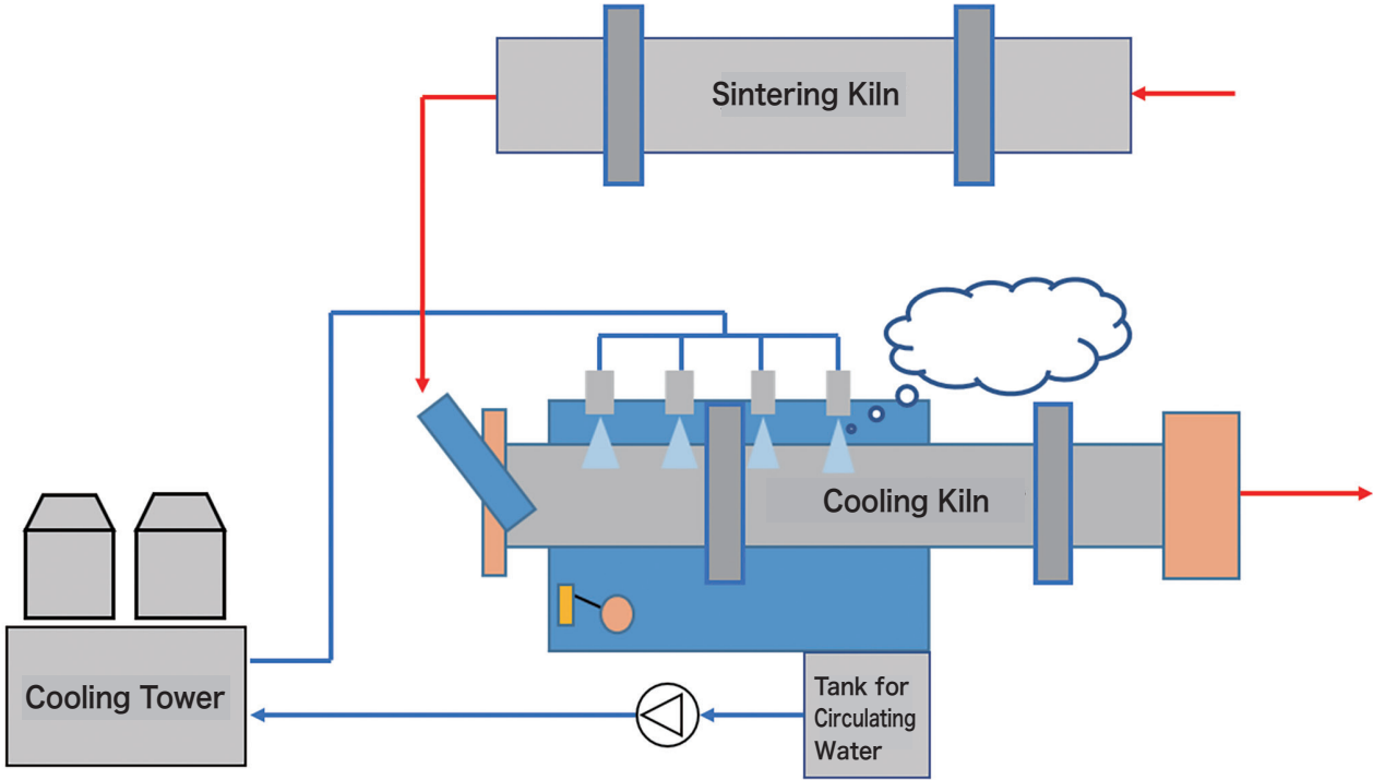
Figure 3-1: Flow Diagram of Indirect-Cooling Kiln Technique
